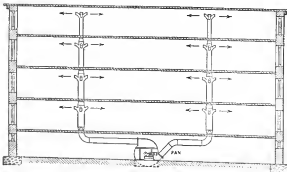
FIG. 3. STAND PIPE SYSTEM OF HEATING AND VENTILATING EMPLOYED IN MULTI-STORY BUILDINGS
